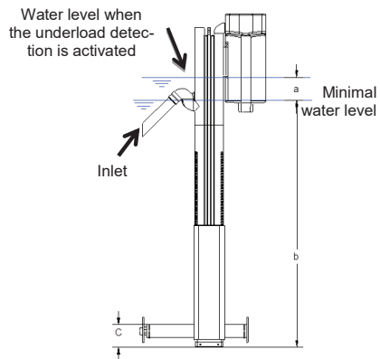
Figure 10– Level measurement via membrane tube aerator
