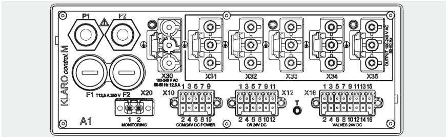
Figure 14 – Electrical connections for KLcontrol.M
