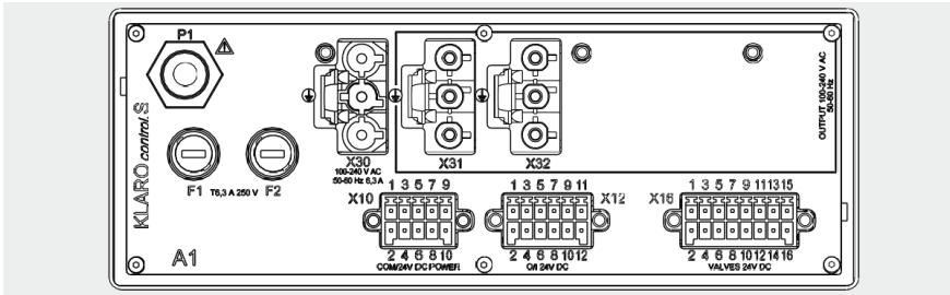
Figure 13 – Electrical connections for KLcontrol.S
