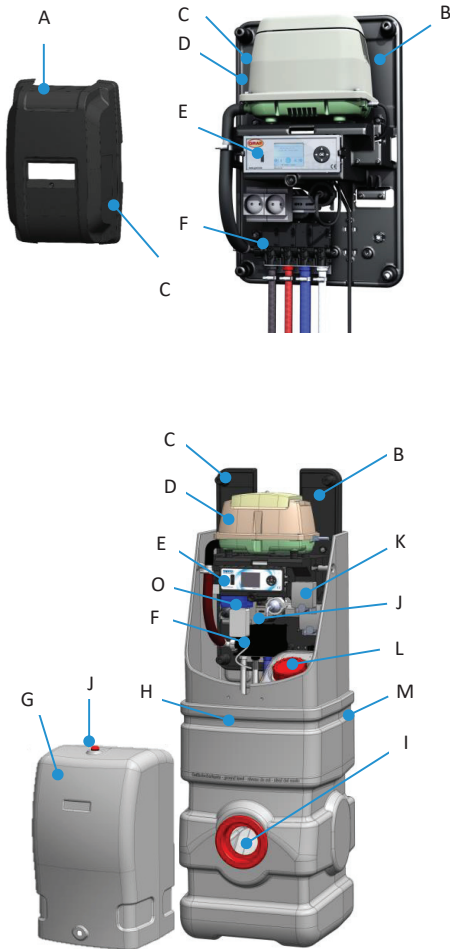
Figure 5 – Example layout of an external switch cabinet for internal PP switch cabinet
