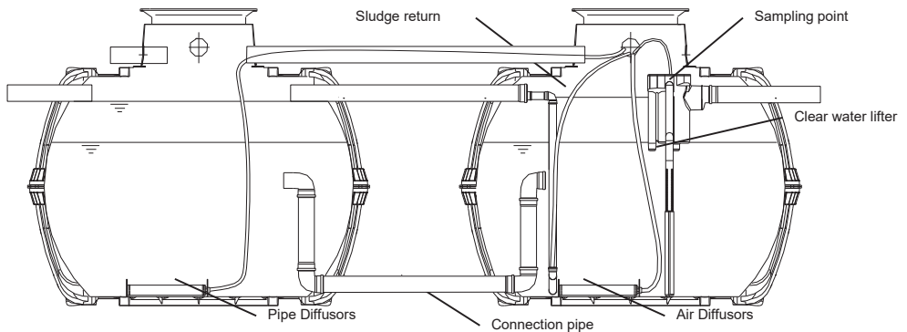
Figure 3 – Example multi tank system in two Carat tanks
