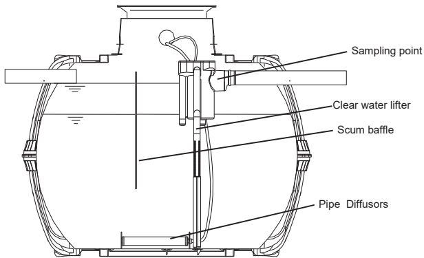
Figure 2 – Example one-tank system in a Carat tank
